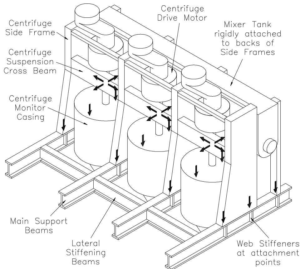
Figure 1 Typical Battery of Batch Centrifuges
