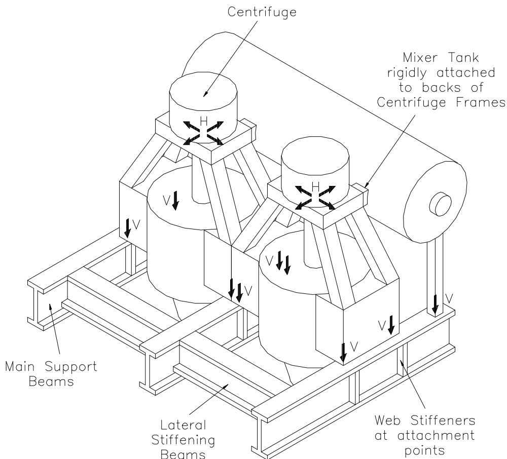
Figure 1 Typical Battery of Batch Centrifuges
